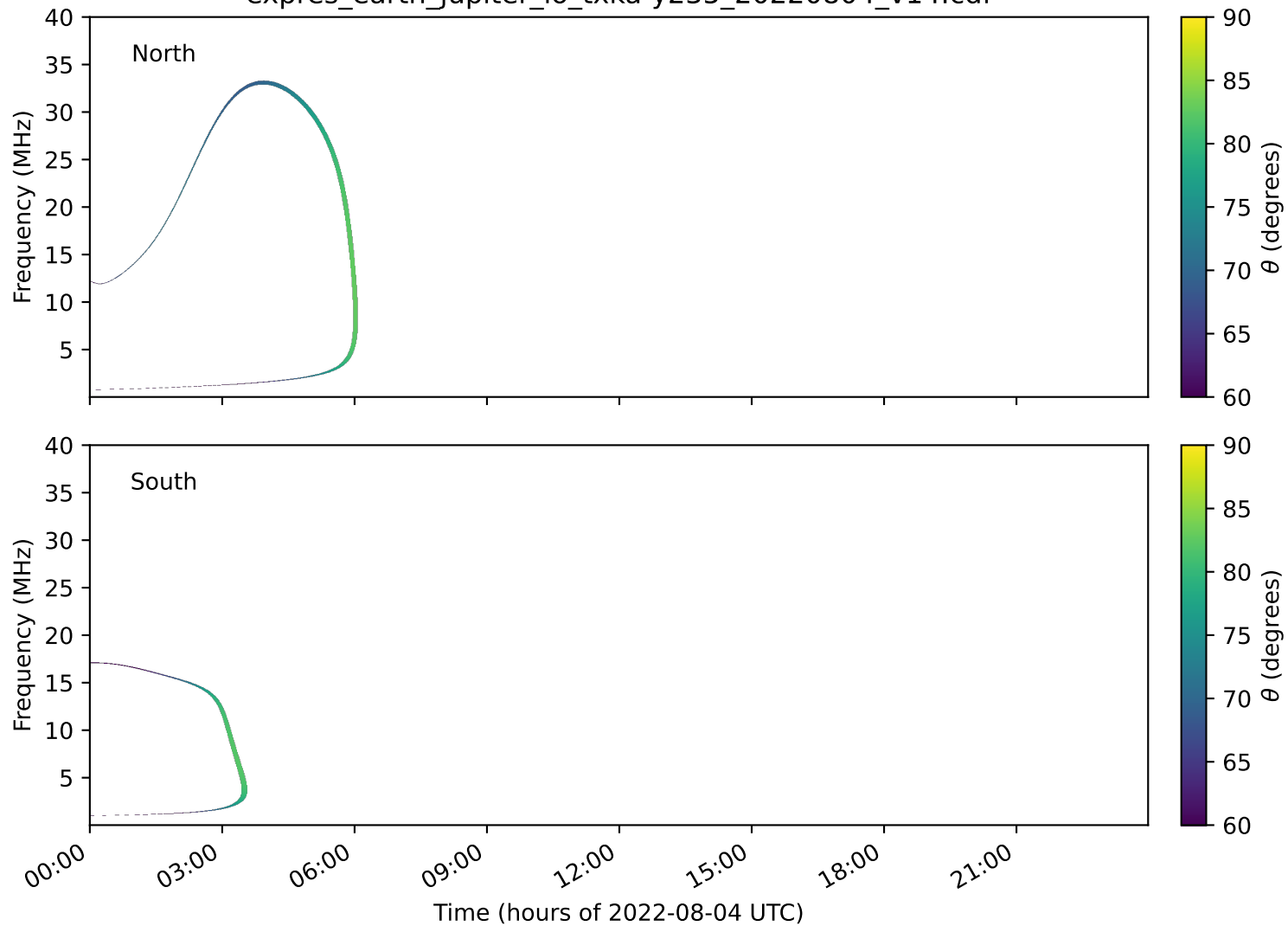
expres_earth_jupiter_io_txka-y235_20220804_v14.cdf
