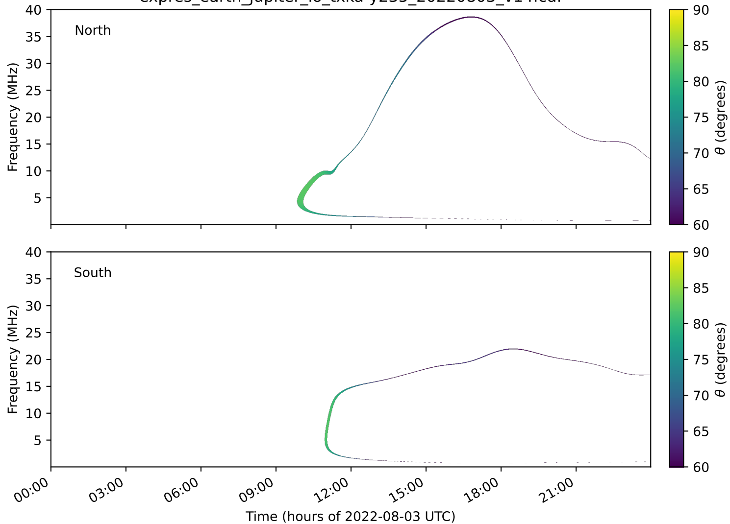
expres_earth_jupiter_io_txka-y235_20220803_v14.cdf
