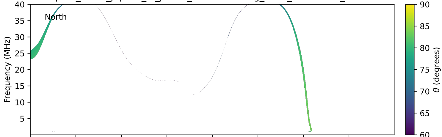
expres_earth_jupiter_io_jrm33_lossc-wid1deg_3kev_20220830_v11.cdf
