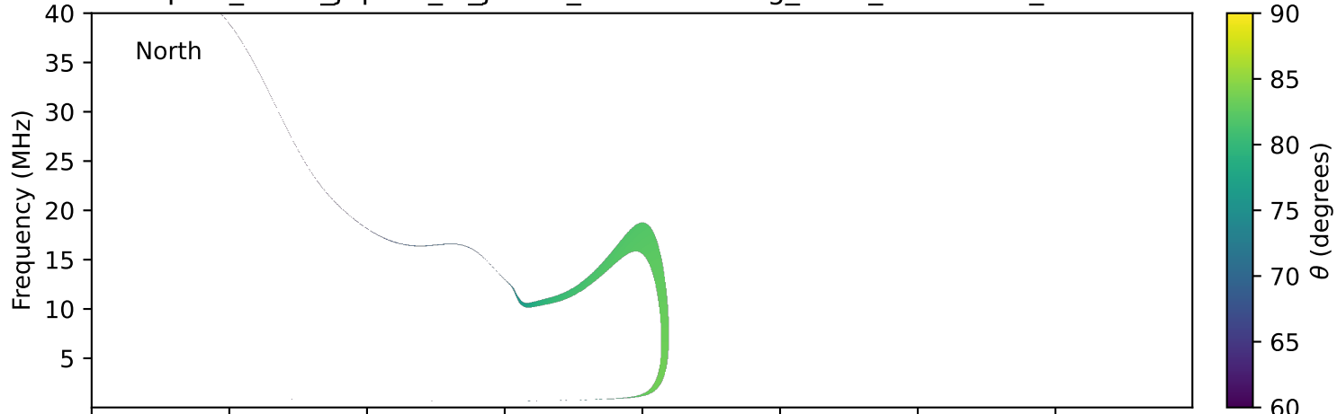
expres_earth_jupiter_io_jrm33_lossc-wid1deg_3kev_20220802_v11.cdf
