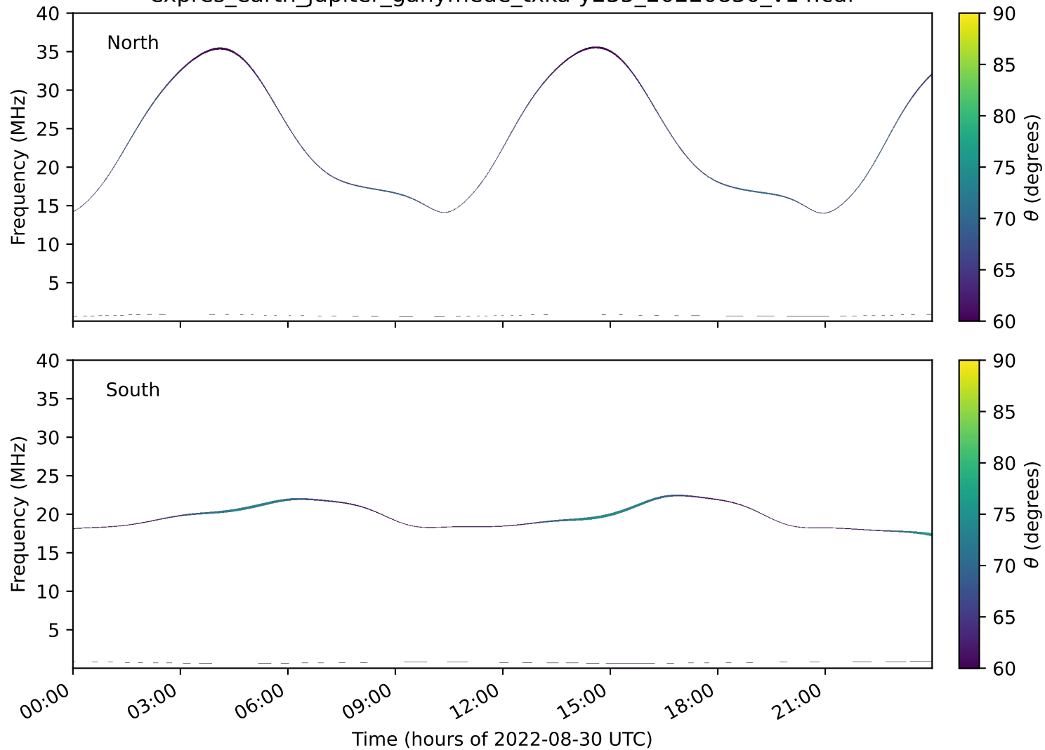
expres_earth_jupiter_ganymede_txka-y235_20220830_v14.cdf
