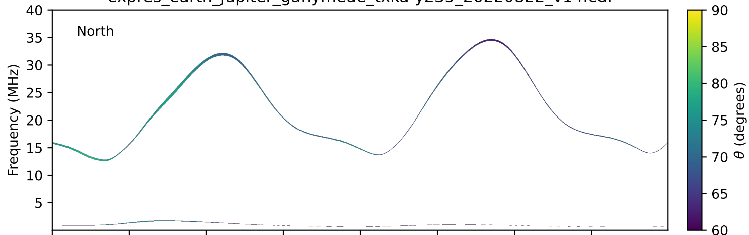
expres_earth_jupiter_ganymede_txka-y235_20220822_v14.cdf
