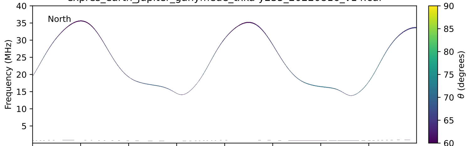
expres_earth_jupiter_ganymede_txka-y235_20220816_v14.cdf
