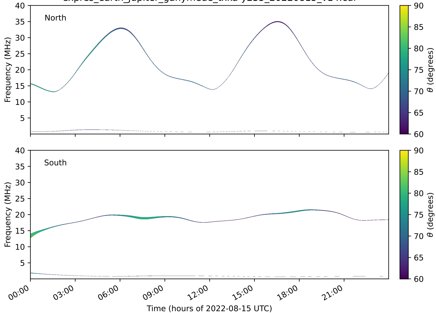
expres_earth_jupiter_ganymede_txka-y235_20220815_v14.cdf
