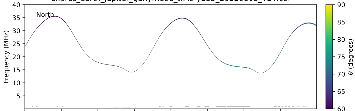
expres_earth_jupiter_ganymede_txka-y235_20220809_v14.cdf
