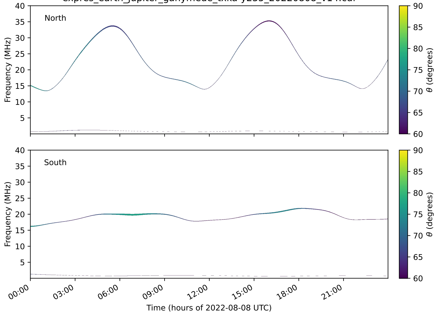
expres_earth_jupiter_ganymede_txka-y235_20220808_v14.cdf
