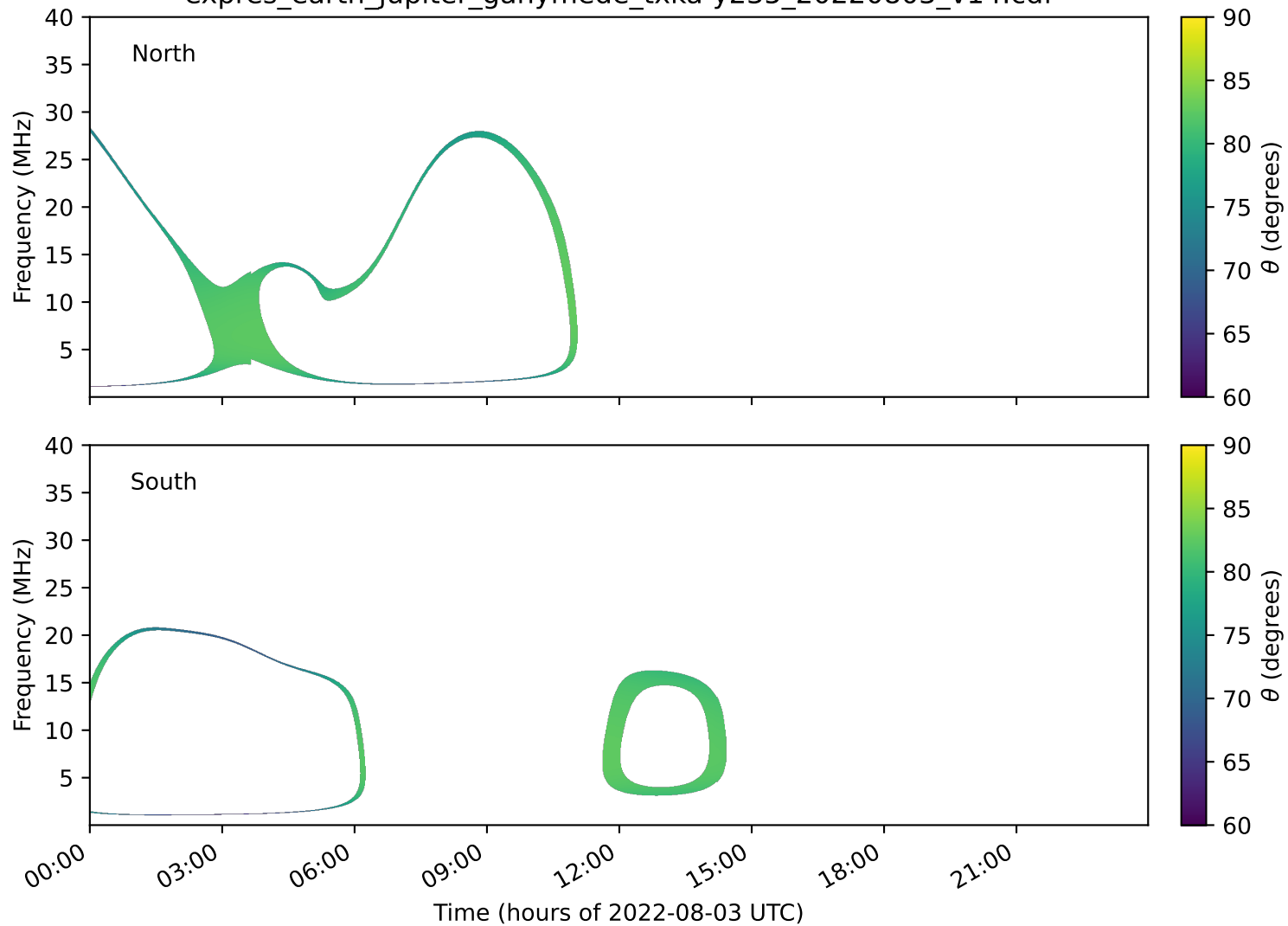
expres_earth_jupiter_ganymede_txka-y235_20220803_v14.cdf
