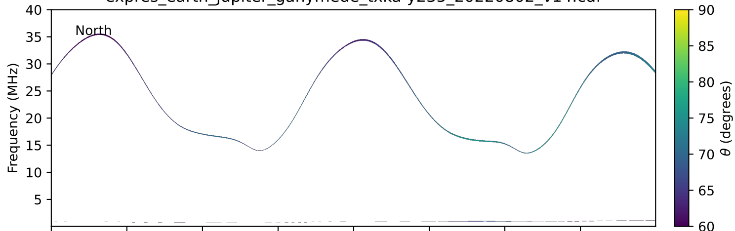
expres_earth_jupiter_ganymede_txka-y235_20220802_v14.cdf
