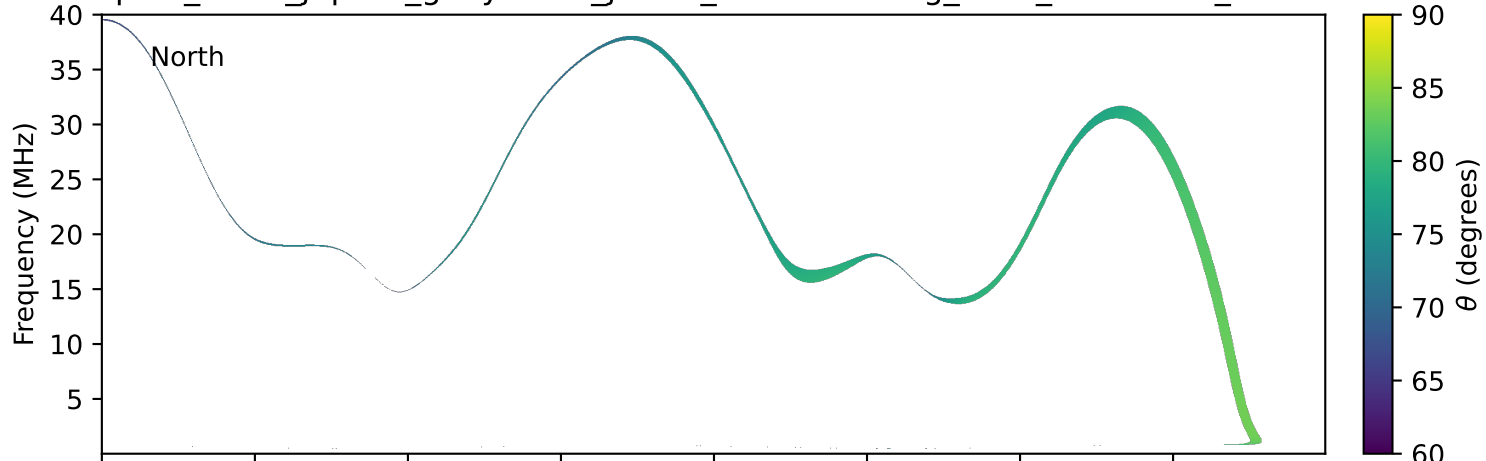
expres_earth_jupiter_ganymede_jrm33_lossc-wid1deg_3kev_20220817_v11.cdf
