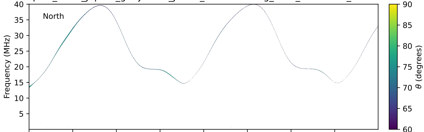
expres_earth_jupiter_ganymede_jrm33_lossc-wid1deg_3kev_20220801_v11.cdf
