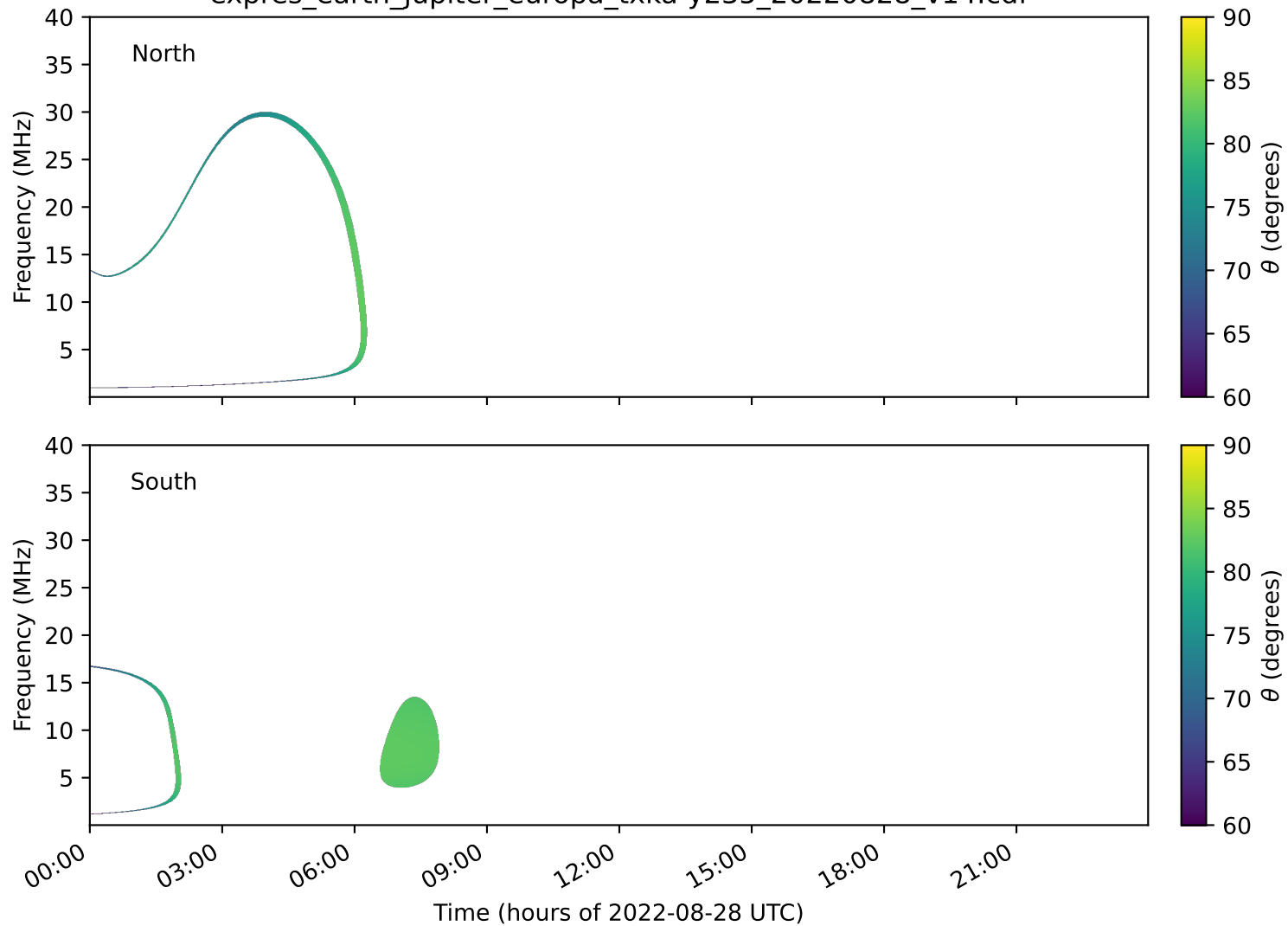
expres_earth_jupiter_europa_txka-y235_20220828_v14.cdf
