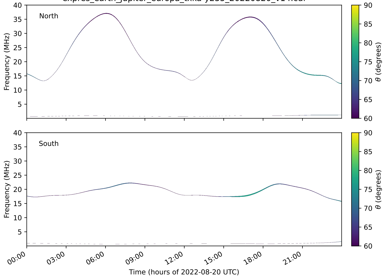
expres_earth_jupiter_europa_txka-y235_20220820_v14.cdf
