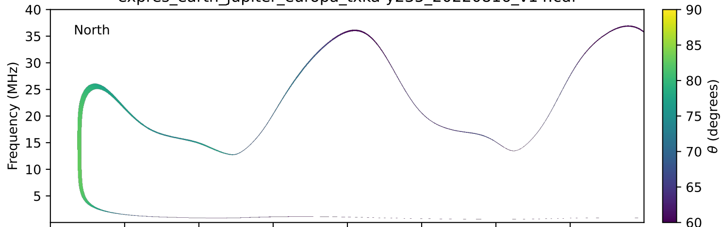
expres_earth_jupiter_europa_txka-y235_20220816_v14.cdf
