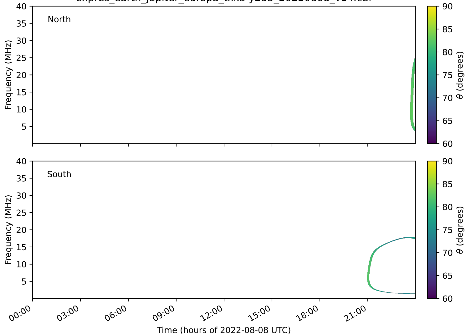
expres_earth_jupiter_europa_txka-y235_20220808_v14.cdf
