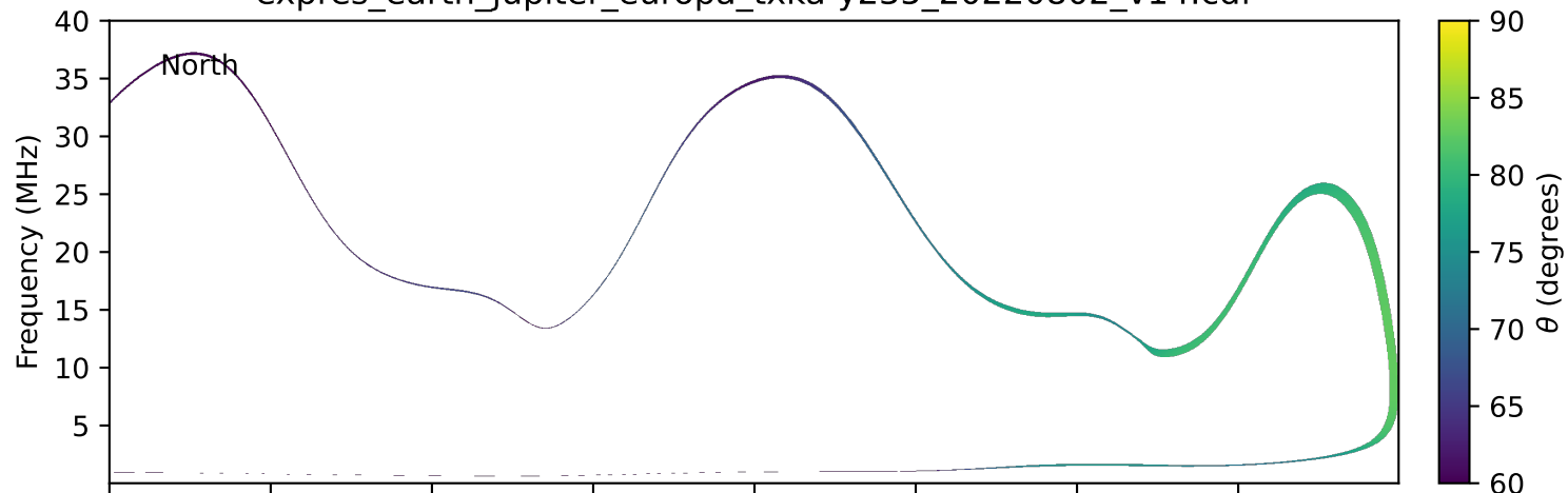
expres_earth_jupiter_europa_txka-y235_20220802_v14.cdf
