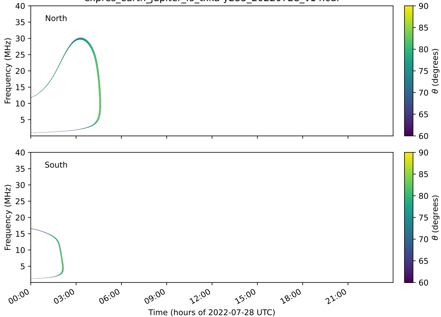
expres_earth_jupiter_io_txka-y235_20220728_v14.cdf
