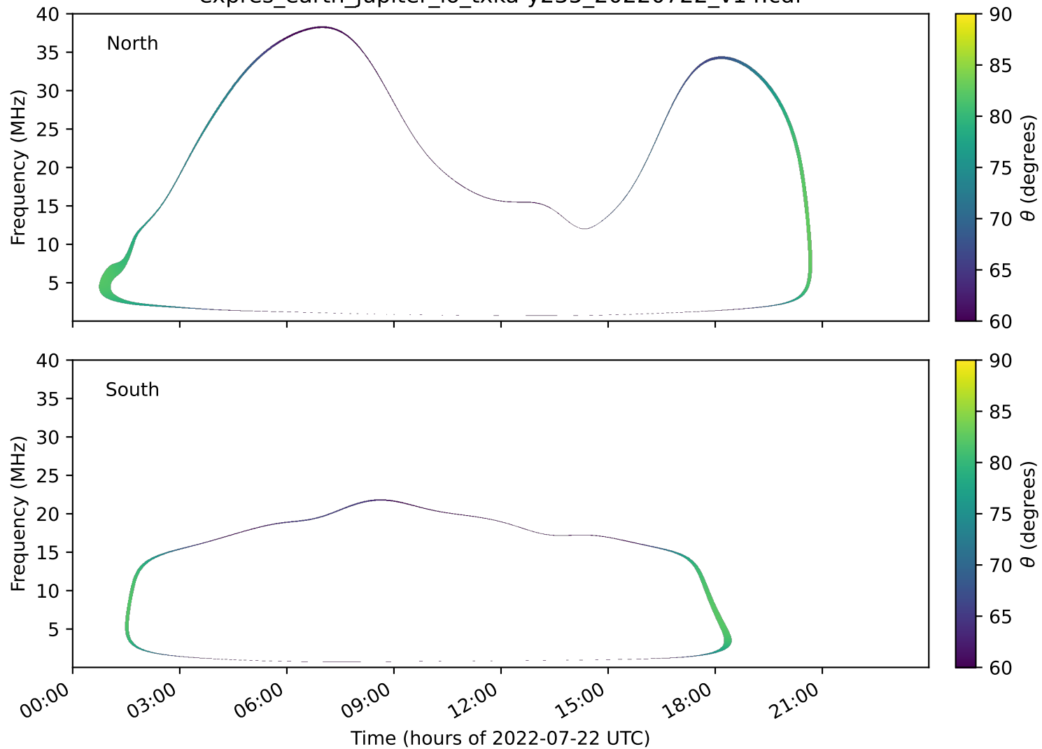
expres_earth_jupiter_io_txka-y235_20220722_v14.cdf
