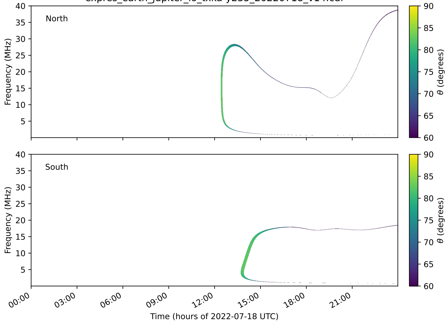
expres_earth_jupiter_io_txka-y235_20220718_v14.cdf
