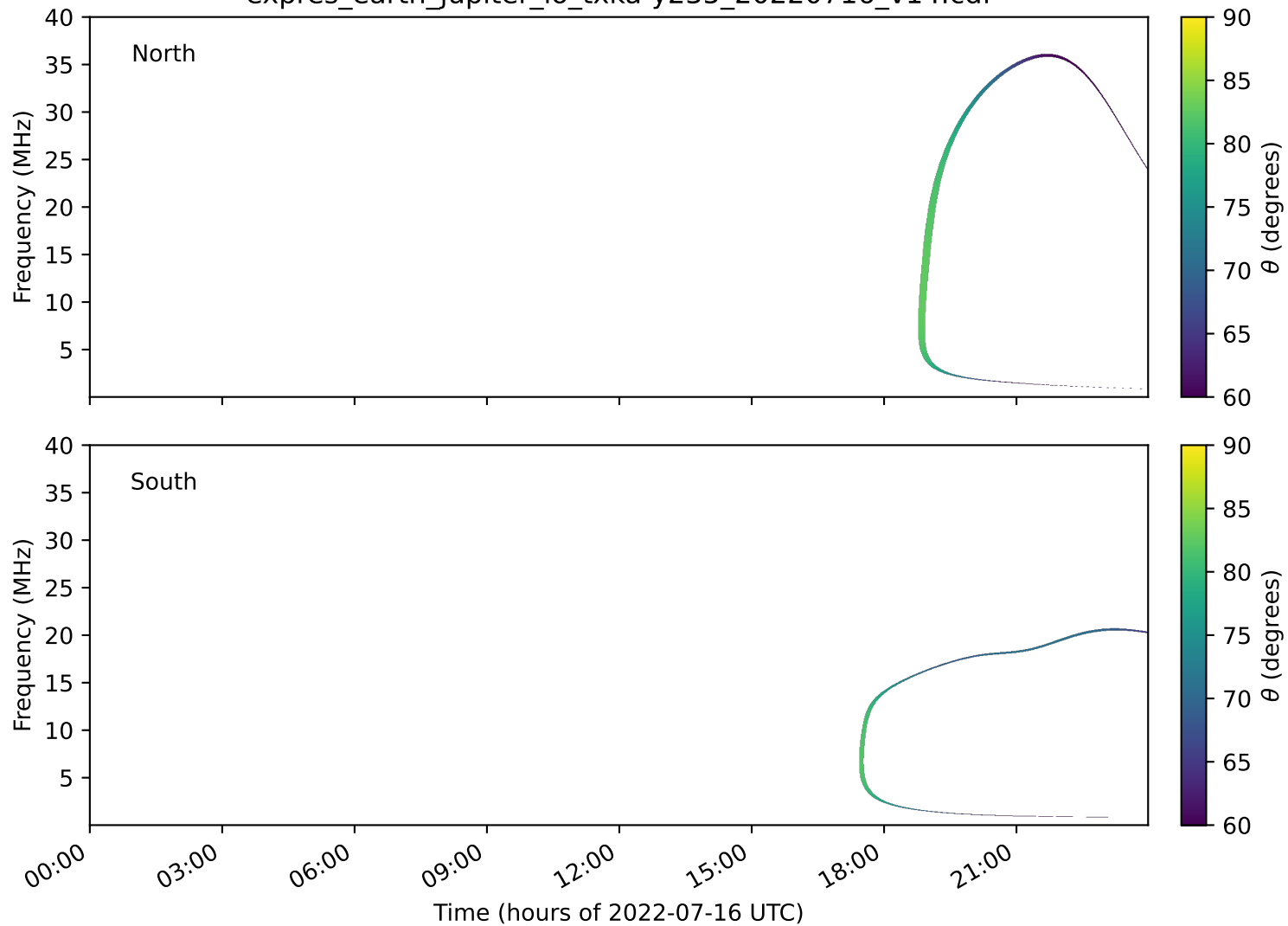
expres_earth_jupiter_io_txka-y235_20220716_v14.cdf
