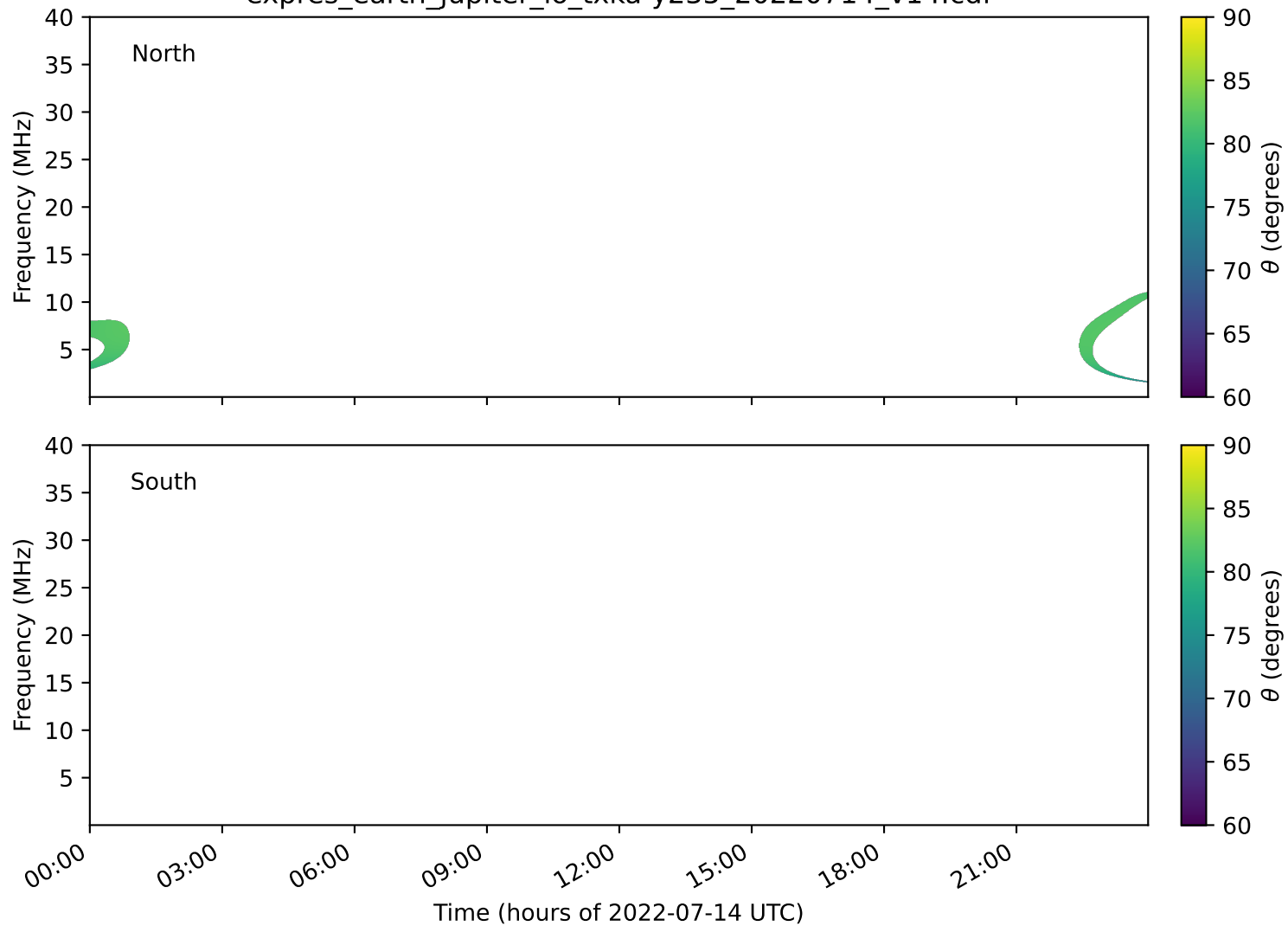
expres_earth_jupiter_io_txka-y235_20220714_v14.cdf
