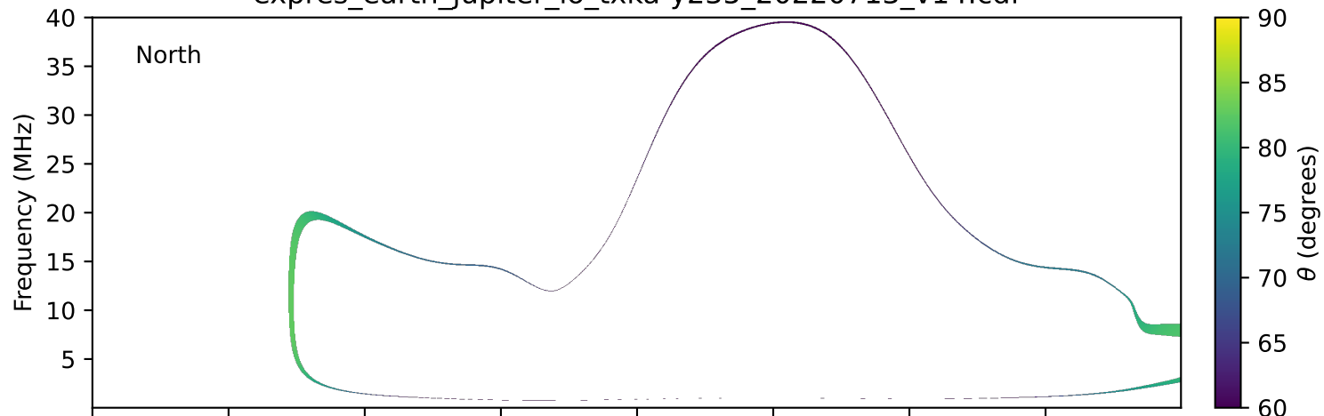
expres_earth_jupiter_io_txka-y235_20220713_v14.cdf
