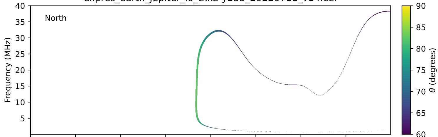
expres_earth_jupiter_io_txka-y235_20220711_v14.cdf
