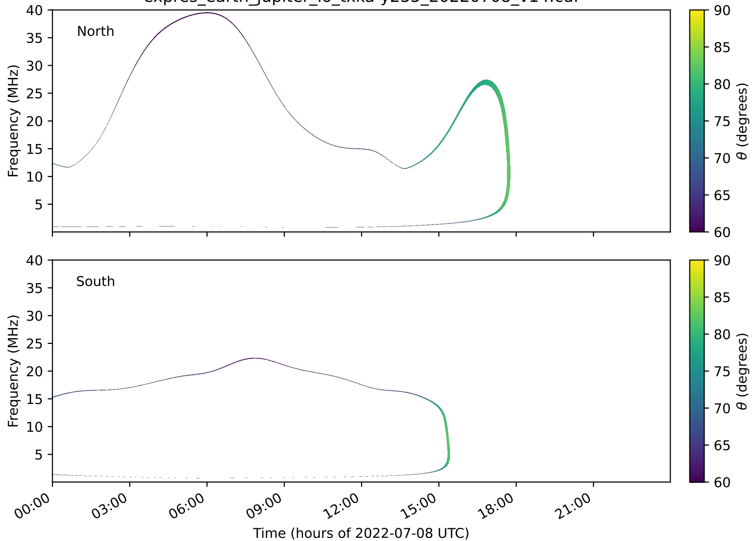
expres_earth_jupiter_io_txka-y235_20220708_v14.cdf
