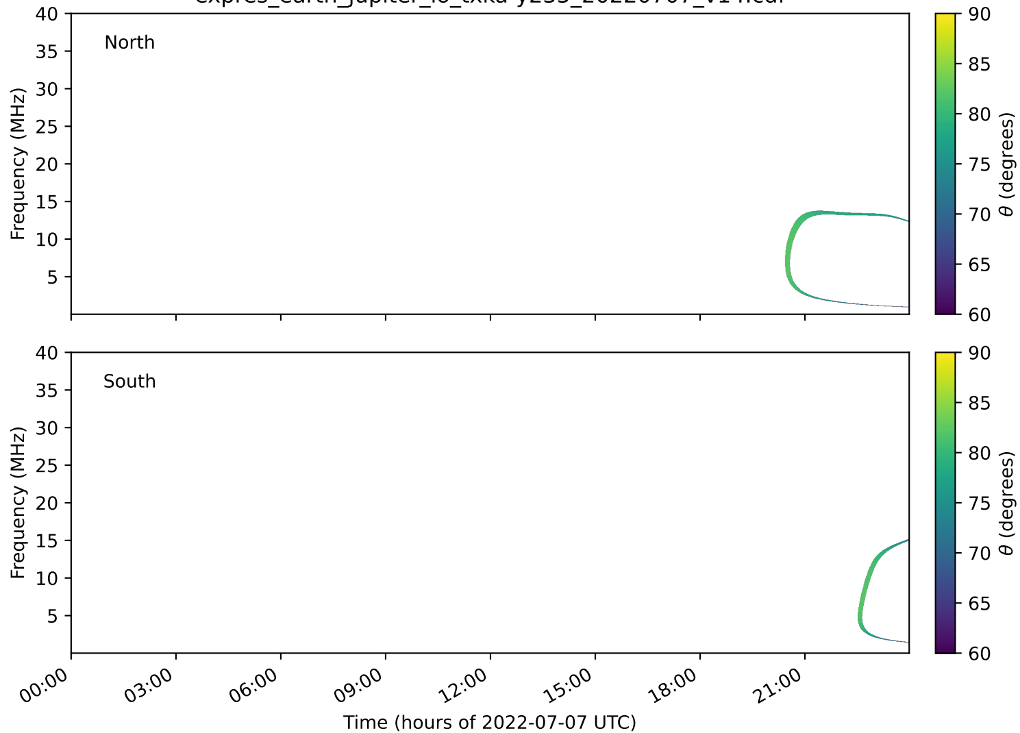
expres_earth_jupiter_io_txka-y235_20220707_v14.cdf
