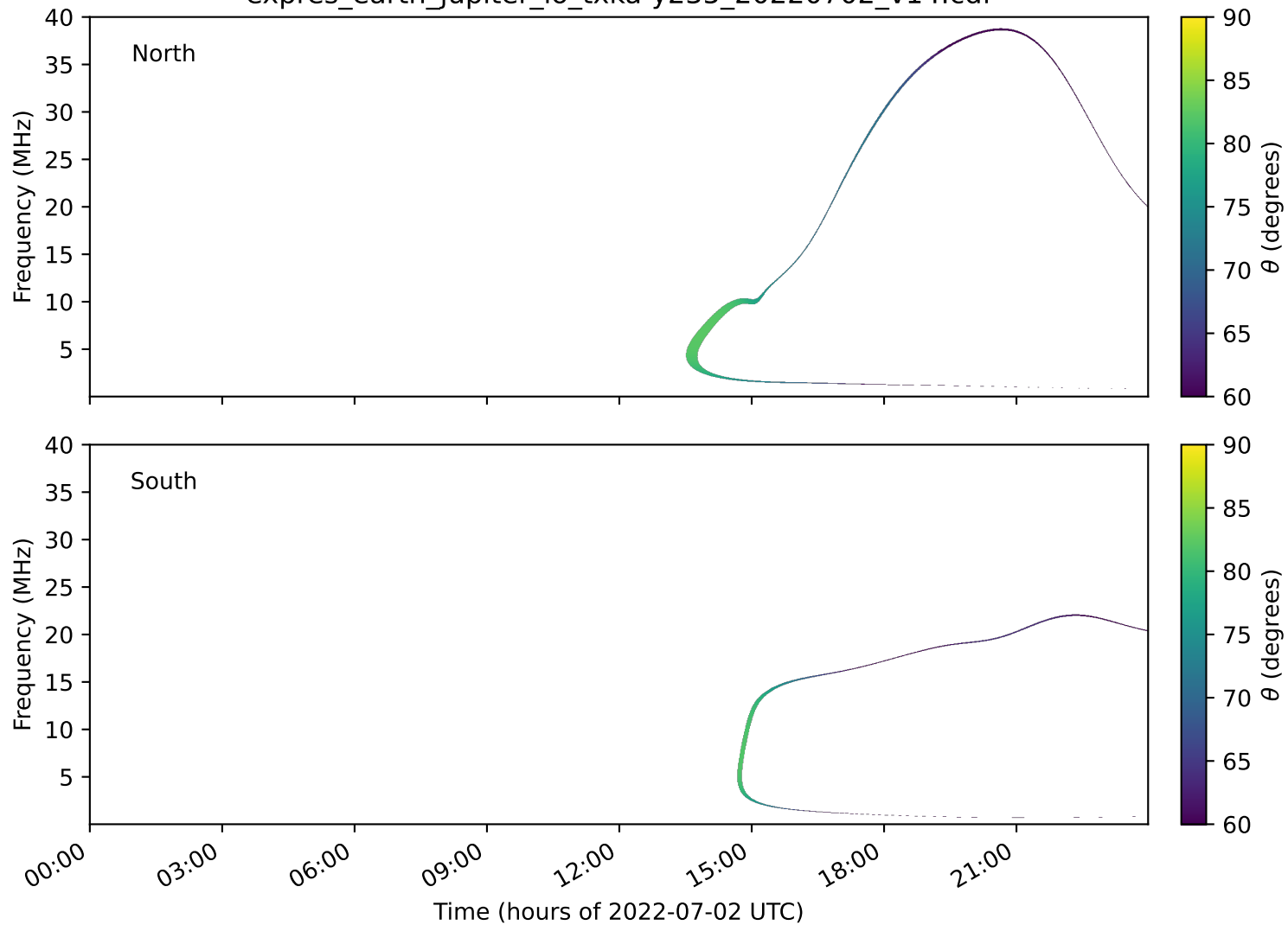
expres_earth_jupiter_io_txka-y235_20220702_v14.cdf
