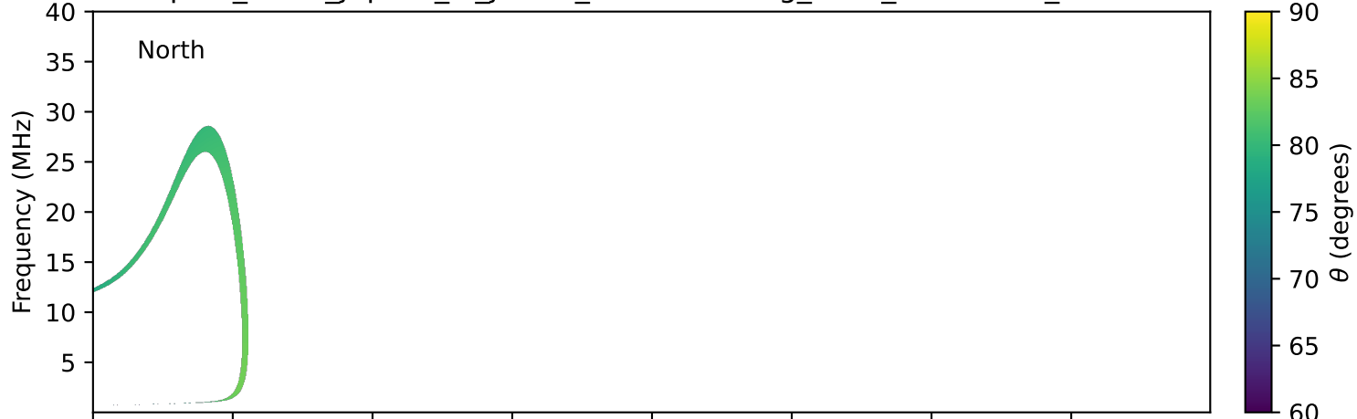
expres_earth_jupiter_io_jrm33_lossc-wid1deg_3kev_20220721_v11.cdf
