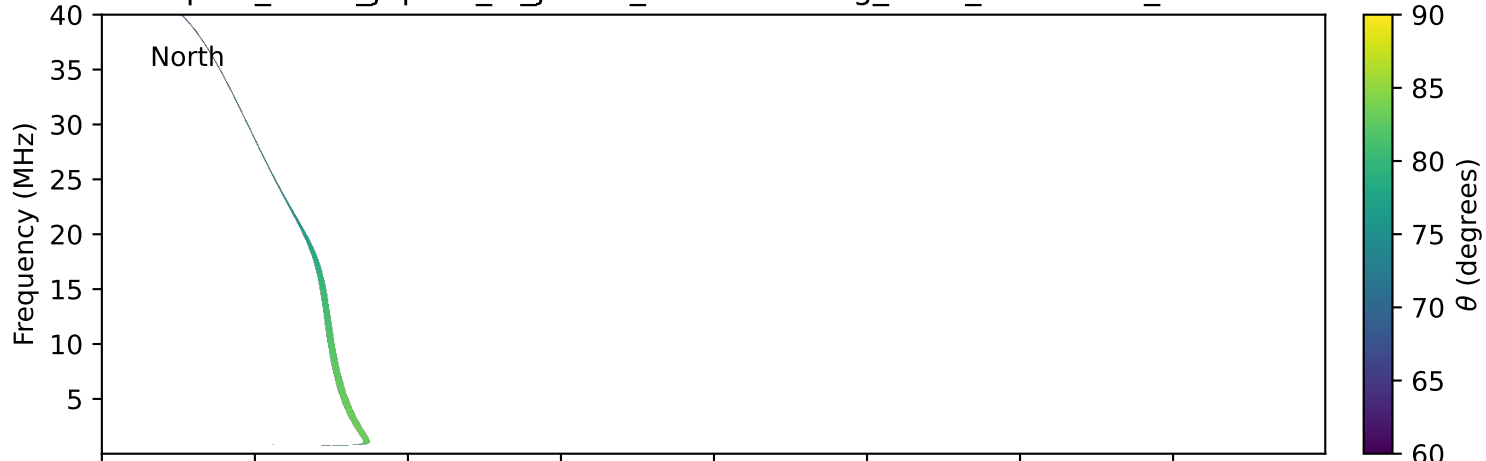
expres_earth_jupiter_io_jrm33_lossc-wid1deg_3kev_20220712_v11.cdf
