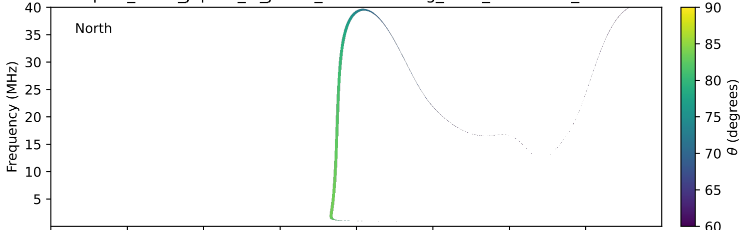
expres_earth_jupiter_io_jrm33_lossc-wid1deg_3kev_20220711_v11.cdf
