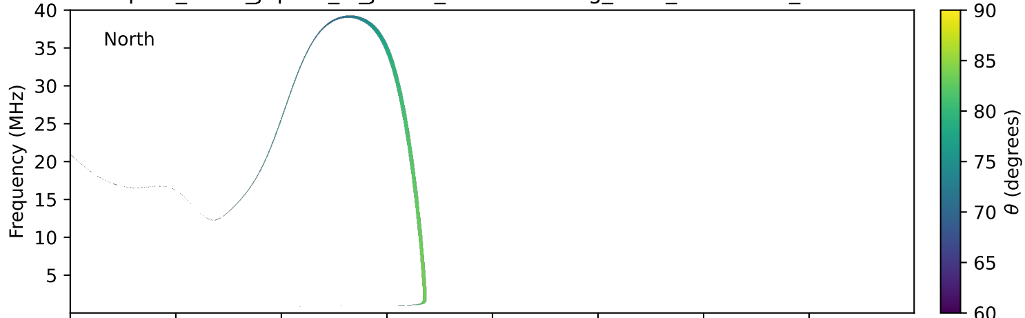
expres_earth_jupiter_io_jrm33_lossc-wid1deg_3kev_20220703_v11.cdf
