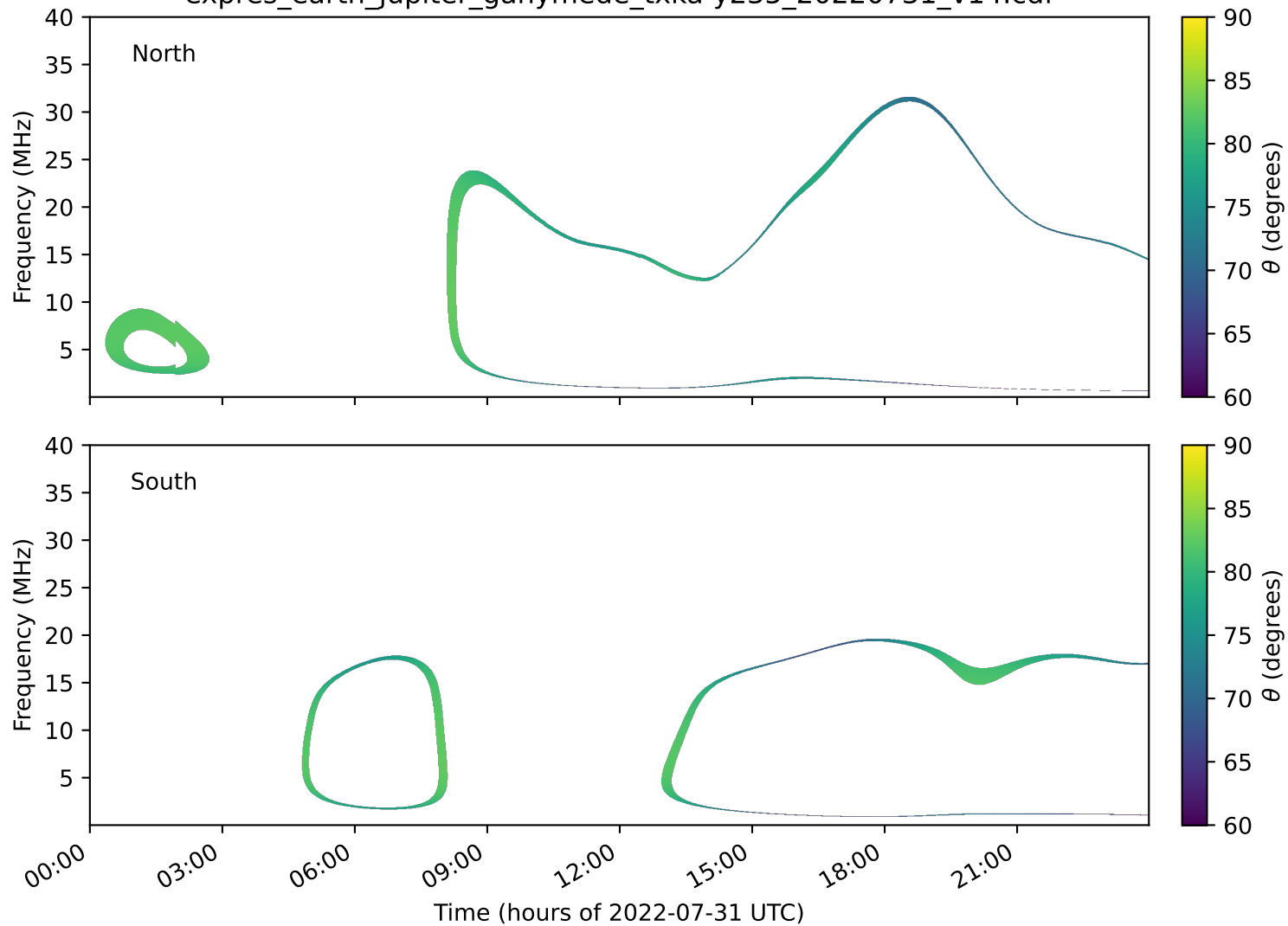
expres_earth_jupiter_ganymede_txka-y235_20220731_v14.cdf
