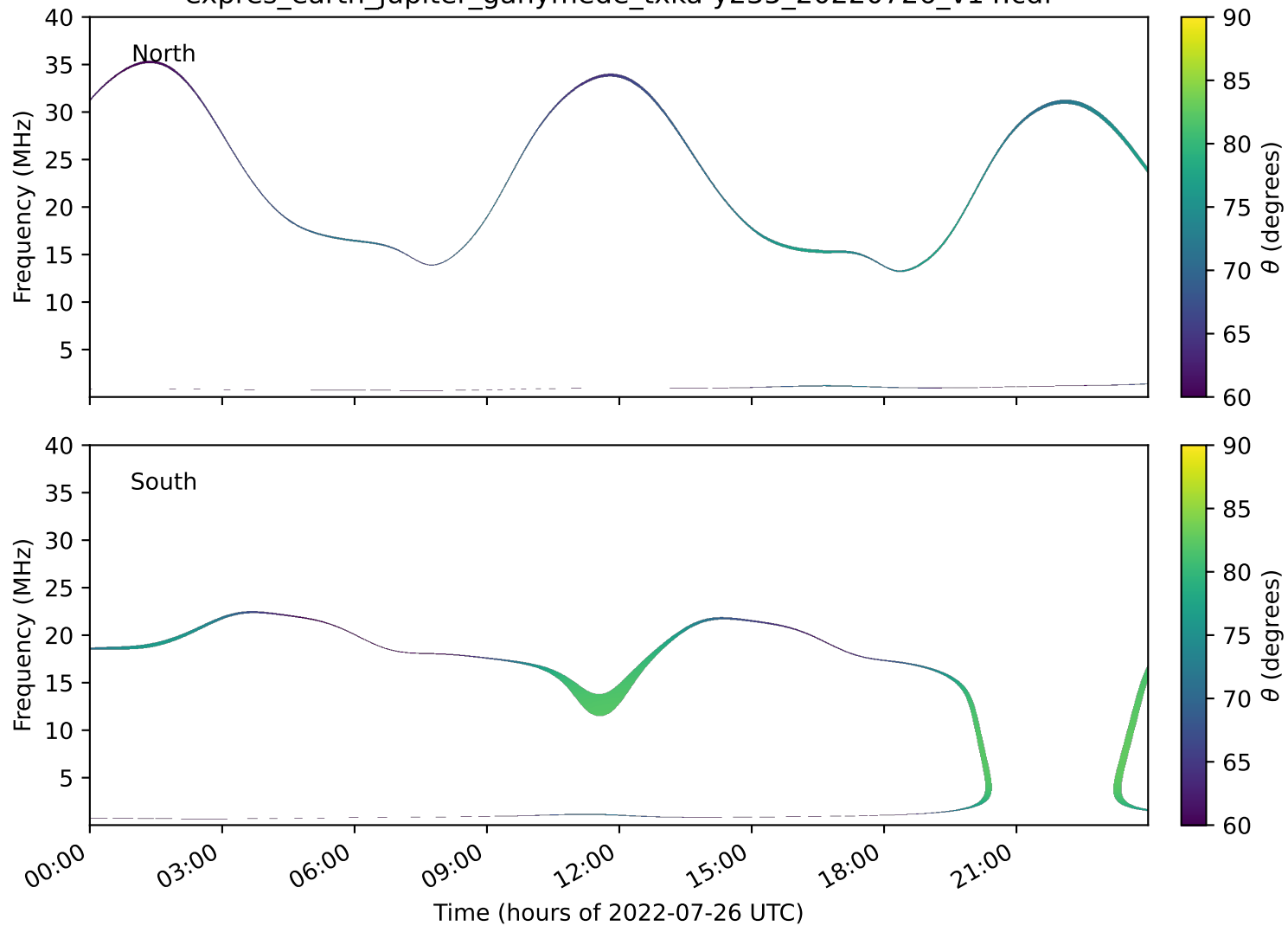
expres_earth_jupiter_ganymede_txka-y235_20220726_v14.cdf
