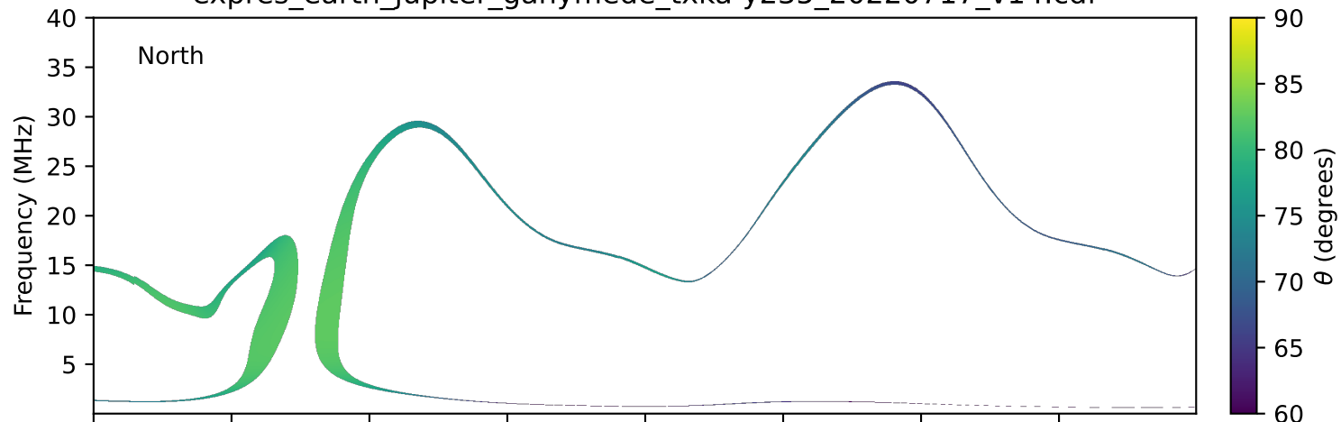
expres_earth_jupiter_ganymede_txka-y235_20220717_v14.cdf
