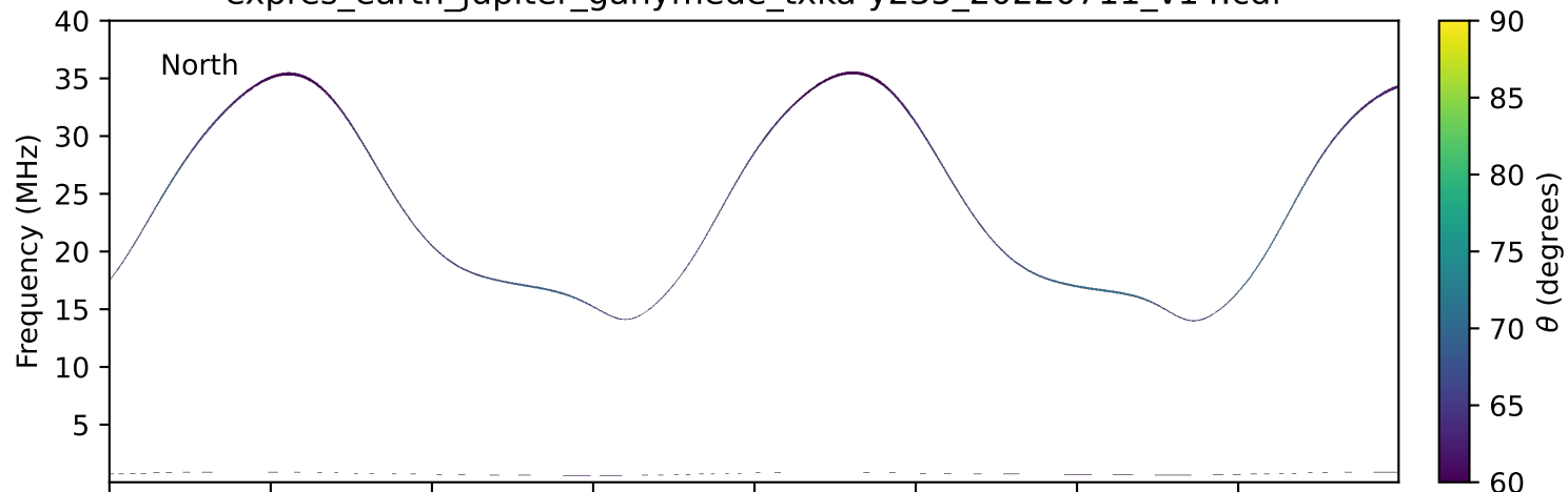
expres_earth_jupiter_ganymede_txka-y235_20220711_v14.cdf
