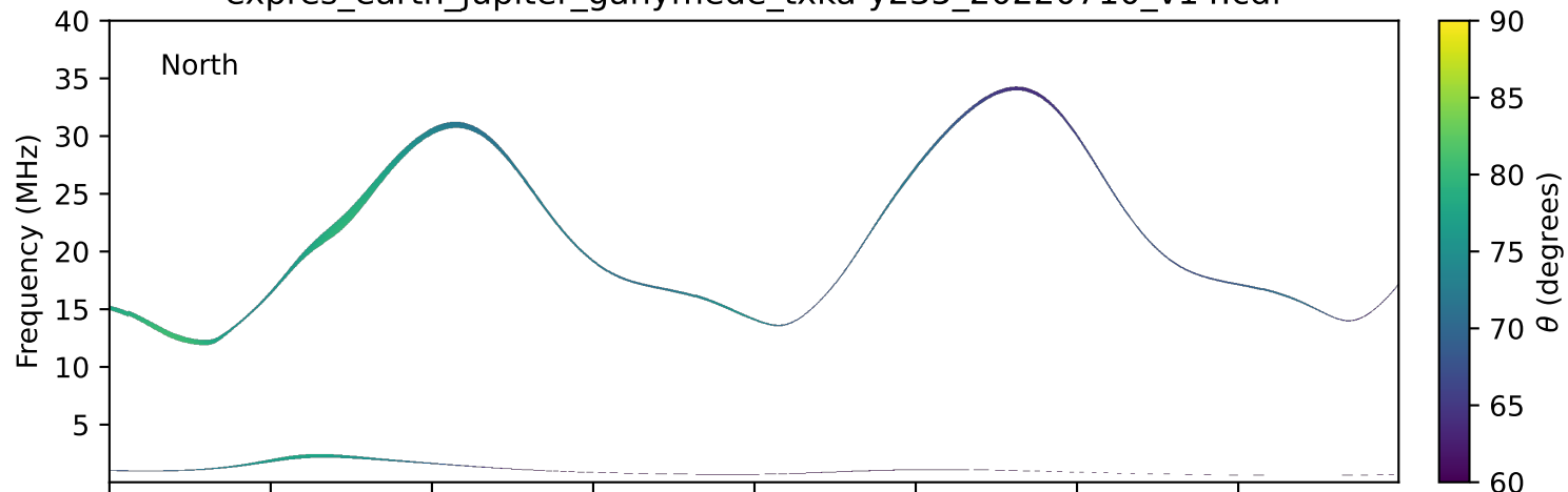
expres_earth_jupiter_ganymede_txka-y235_20220710_v14.cdf
