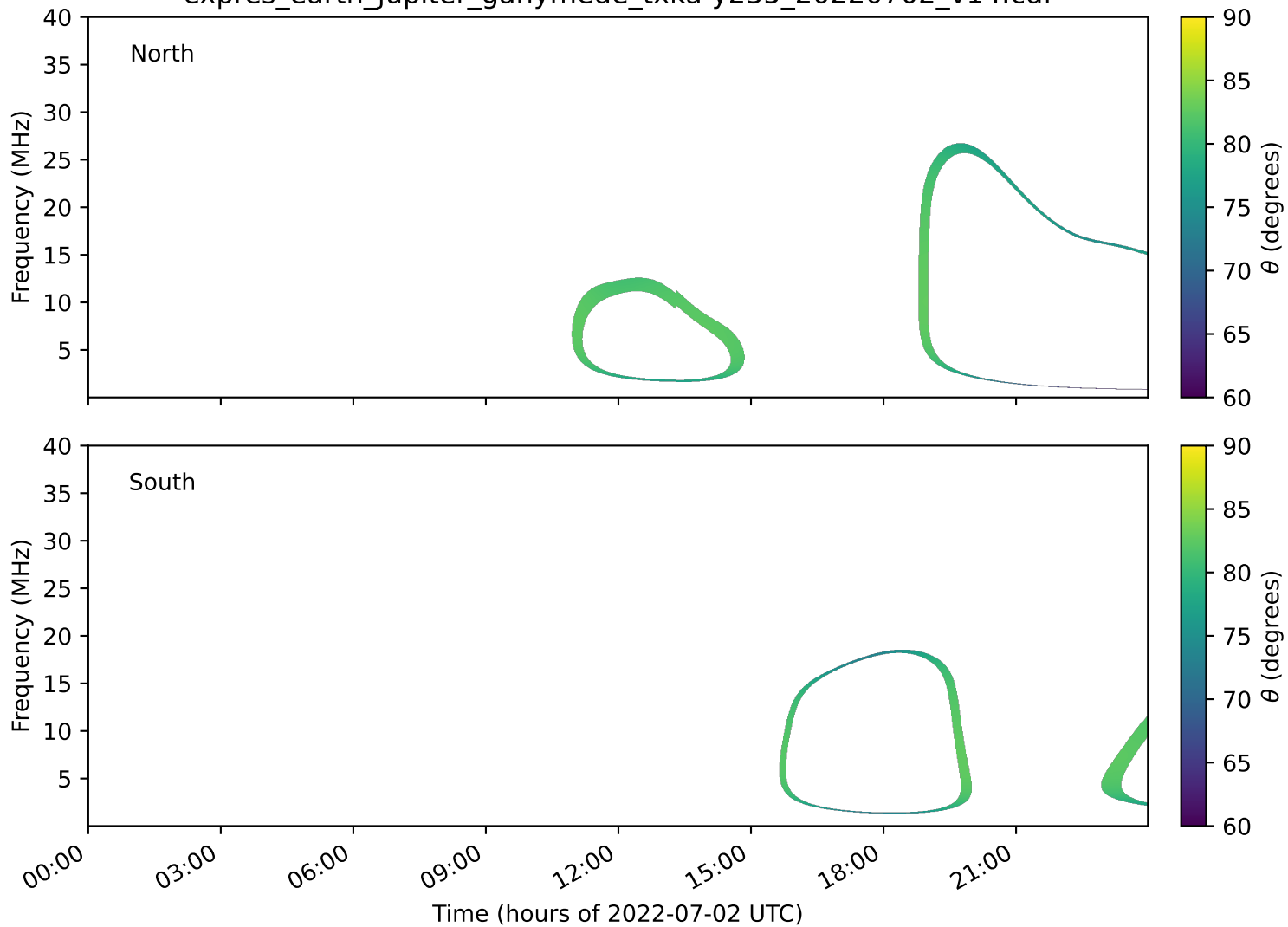
expres_earth_jupiter_ganymede_txka-y235_20220702_v14.cdf
