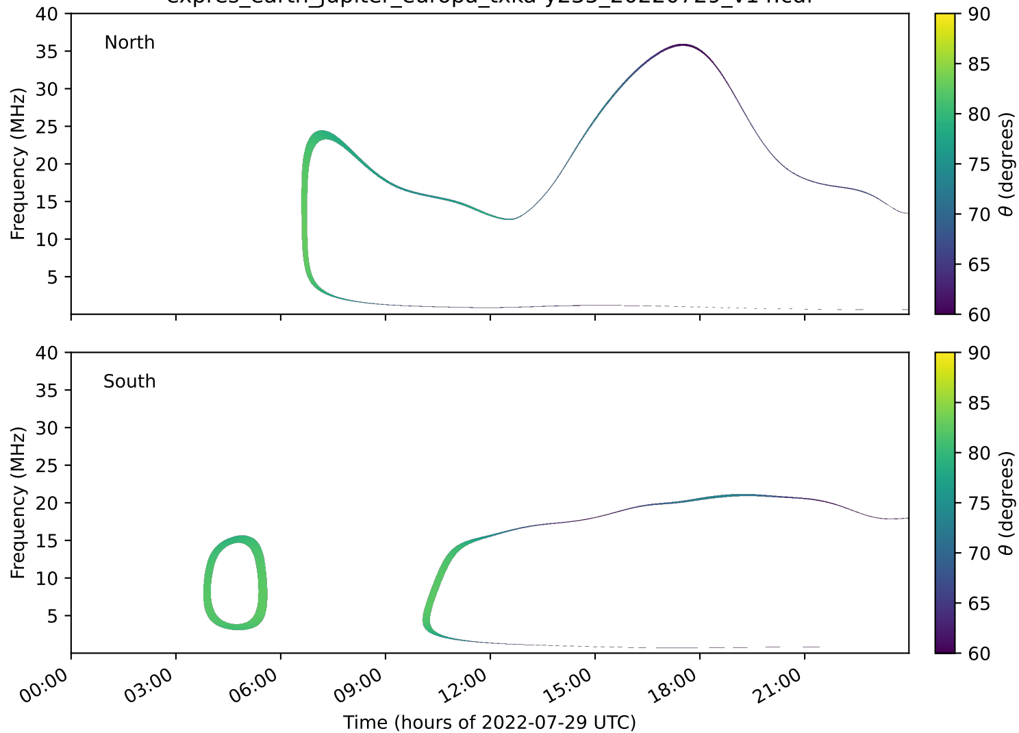
expres_earth_jupiter_europa_txka-y235_20220729_v14.cdf
