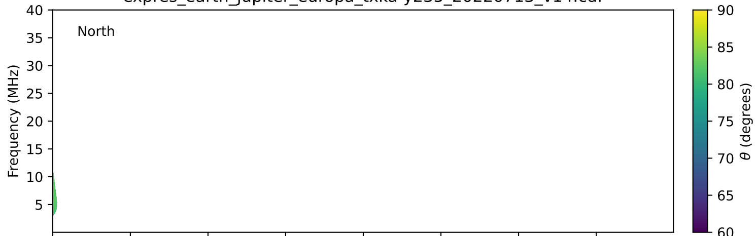
expres_earth_jupiter_europa_txka-y235_20220713_v14.cdf
