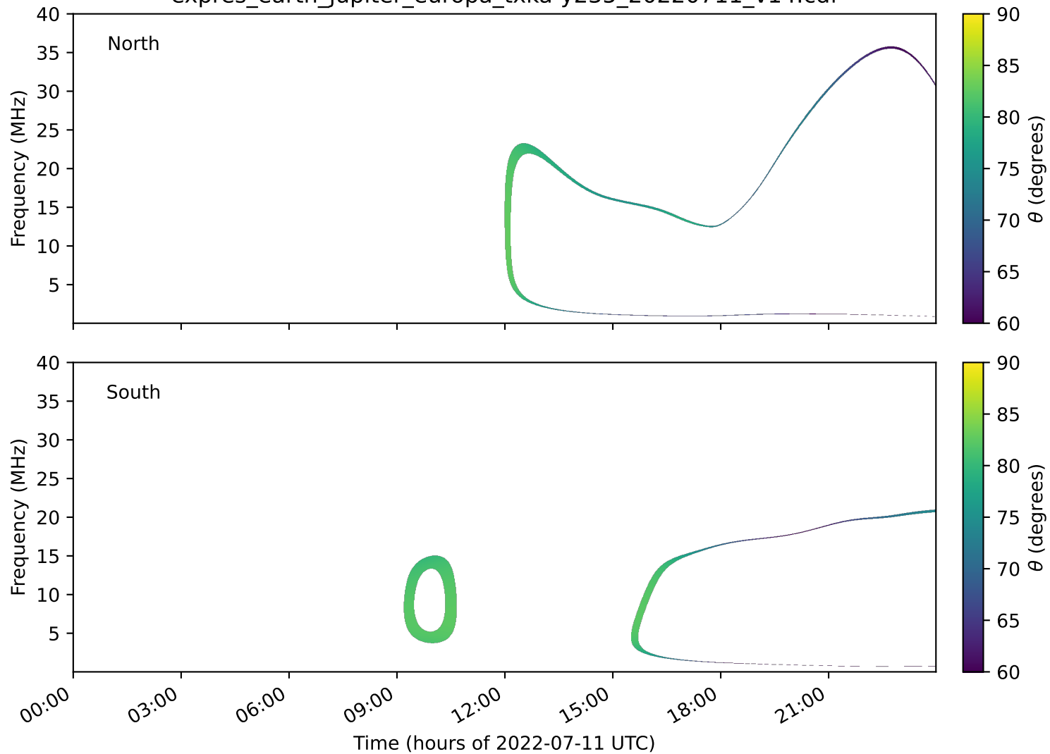
expres_earth_jupiter_europa_txka-y235_20220711_v14.cdf
