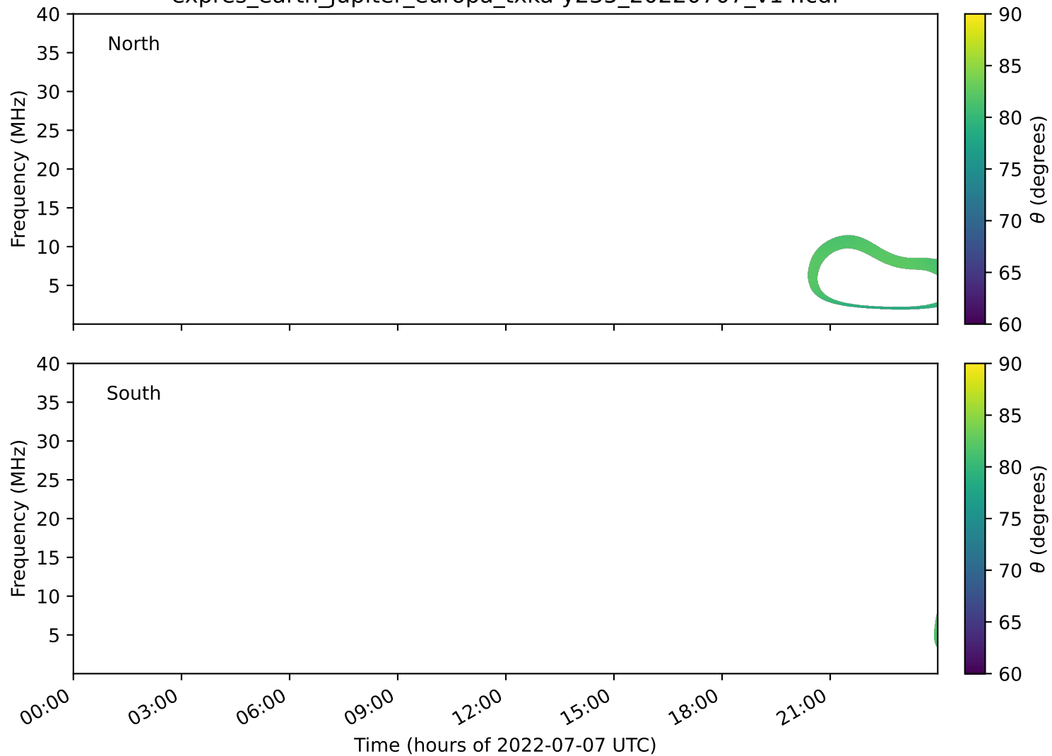
expres_earth_jupiter_europa_txka-y235_20220707_v14.cdf
