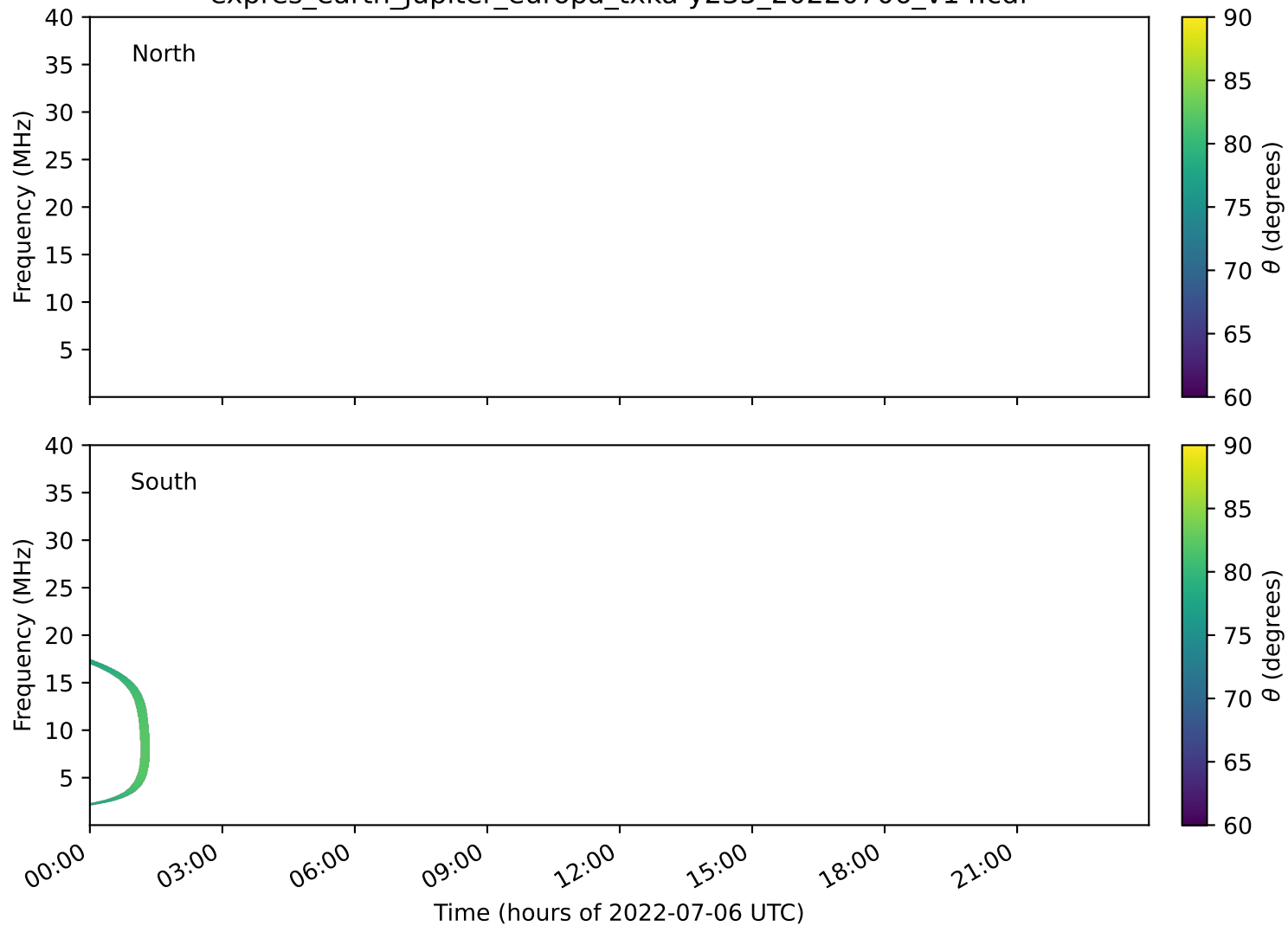
expres_earth_jupiter_europa_txka-y235_20220706_v14.cdf
