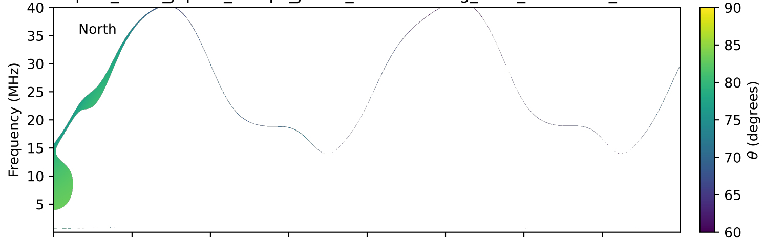
expres_earth_jupiter_europa_jrm33_lossc-wid1deg_3kev_20220701_v11.cdf
