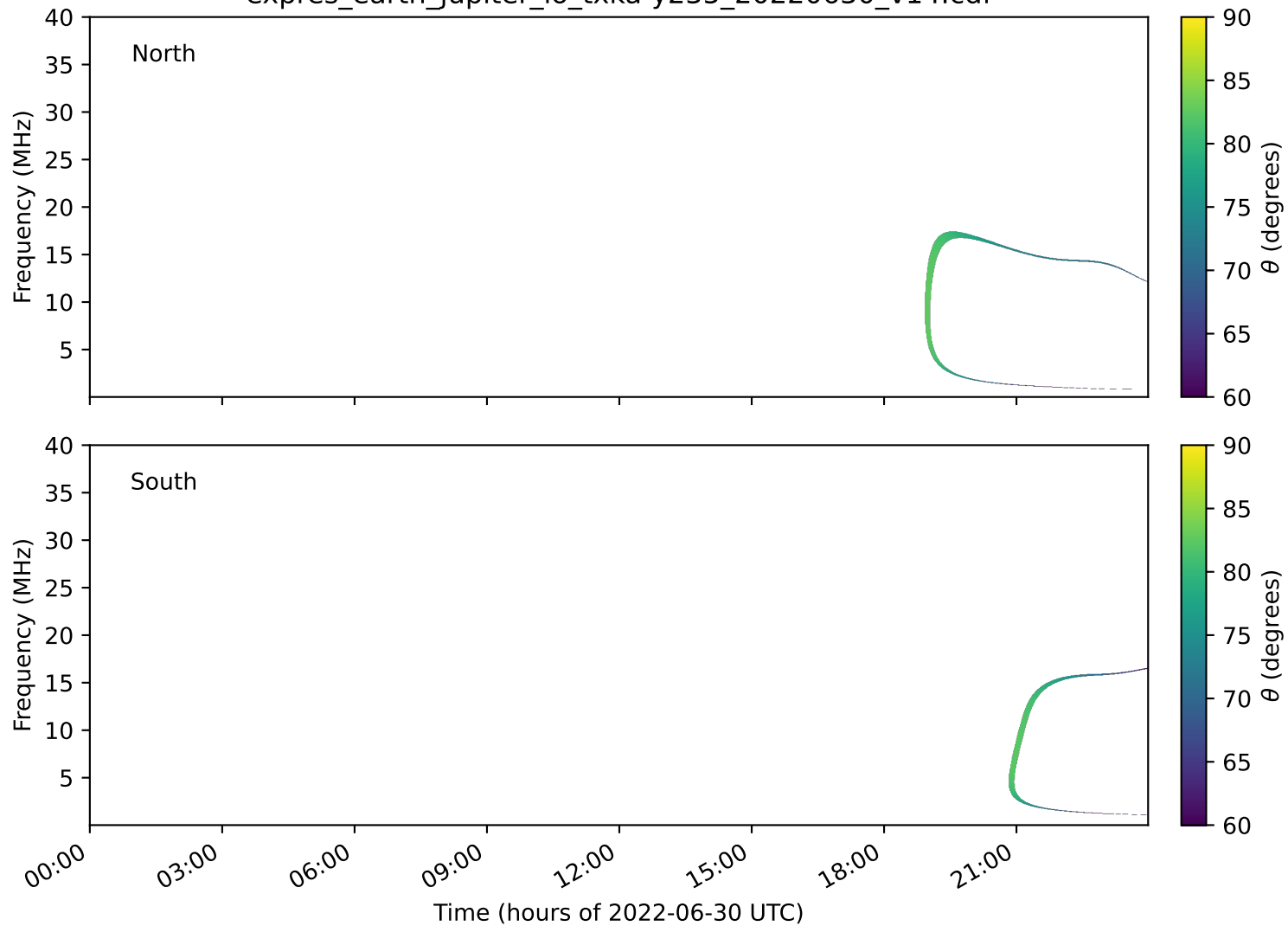
expres_earth_jupiter_io_txka-y235_20220630_v14.cdf
