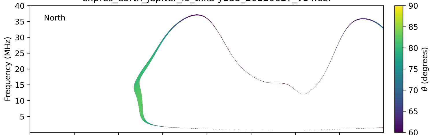
expres_earth_jupiter_io_txka-y235_20220627_v14.cdf
