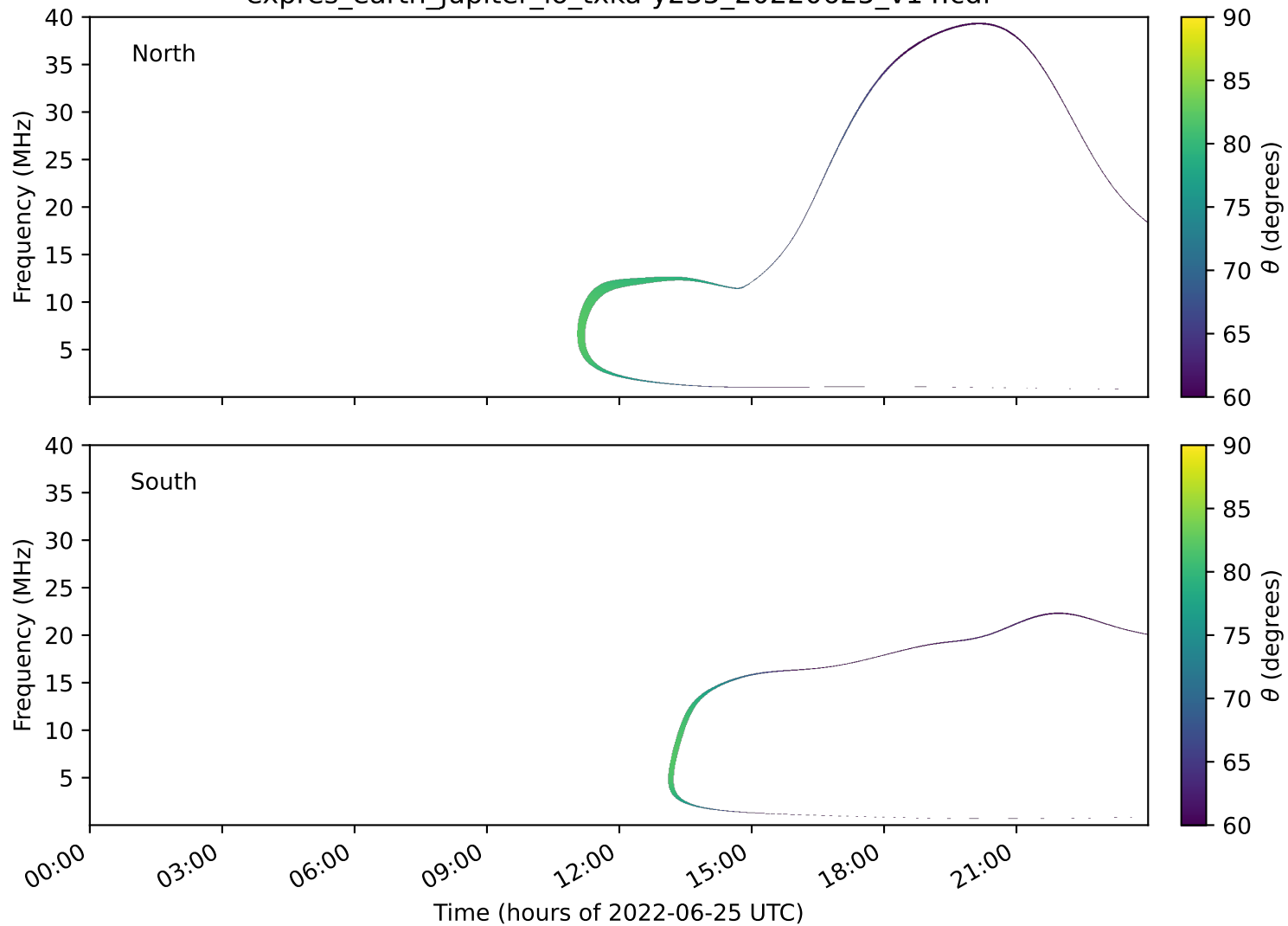
expres_earth_jupiter_io_txka-y235_20220625_v14.cdf
