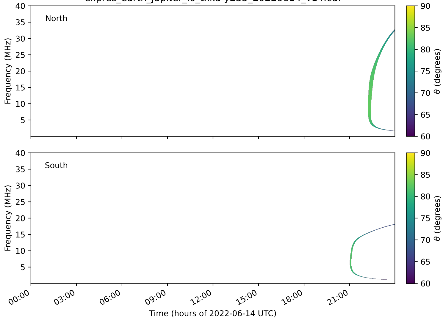
expres_earth_jupiter_io_txka-y235_20220614_v14.cdf
