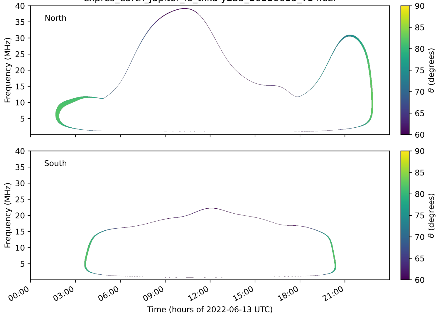
expres_earth_jupiter_io_txka-y235_20220613_v14.cdf
